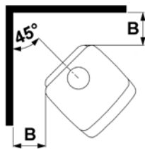
3410 corner installation
