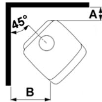
3440 corner installation
