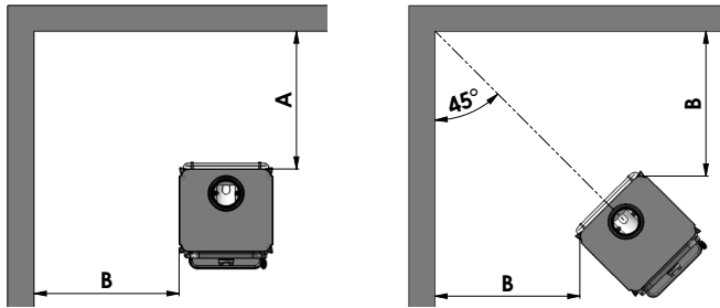
Morsø 1430 corner installation
