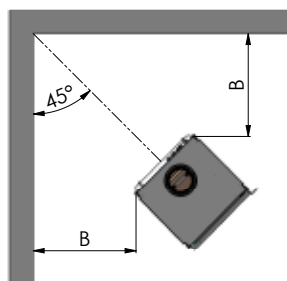
1416/1418 corner installation
