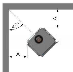
1446/1448 corner installation
