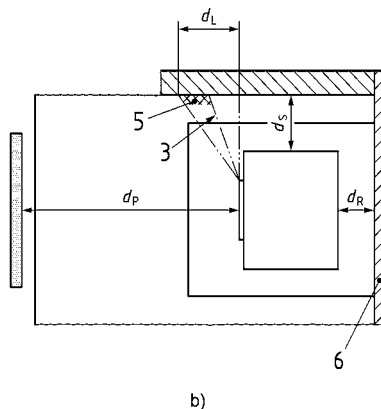
Clearances using insulated flue and exposed flue collar
