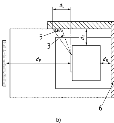
Clearances
